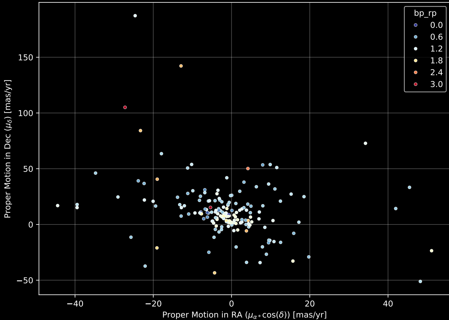
APOGEE DR17 Field: [268-23-O_TESS] Proper Motion Diagram (n= 173)
