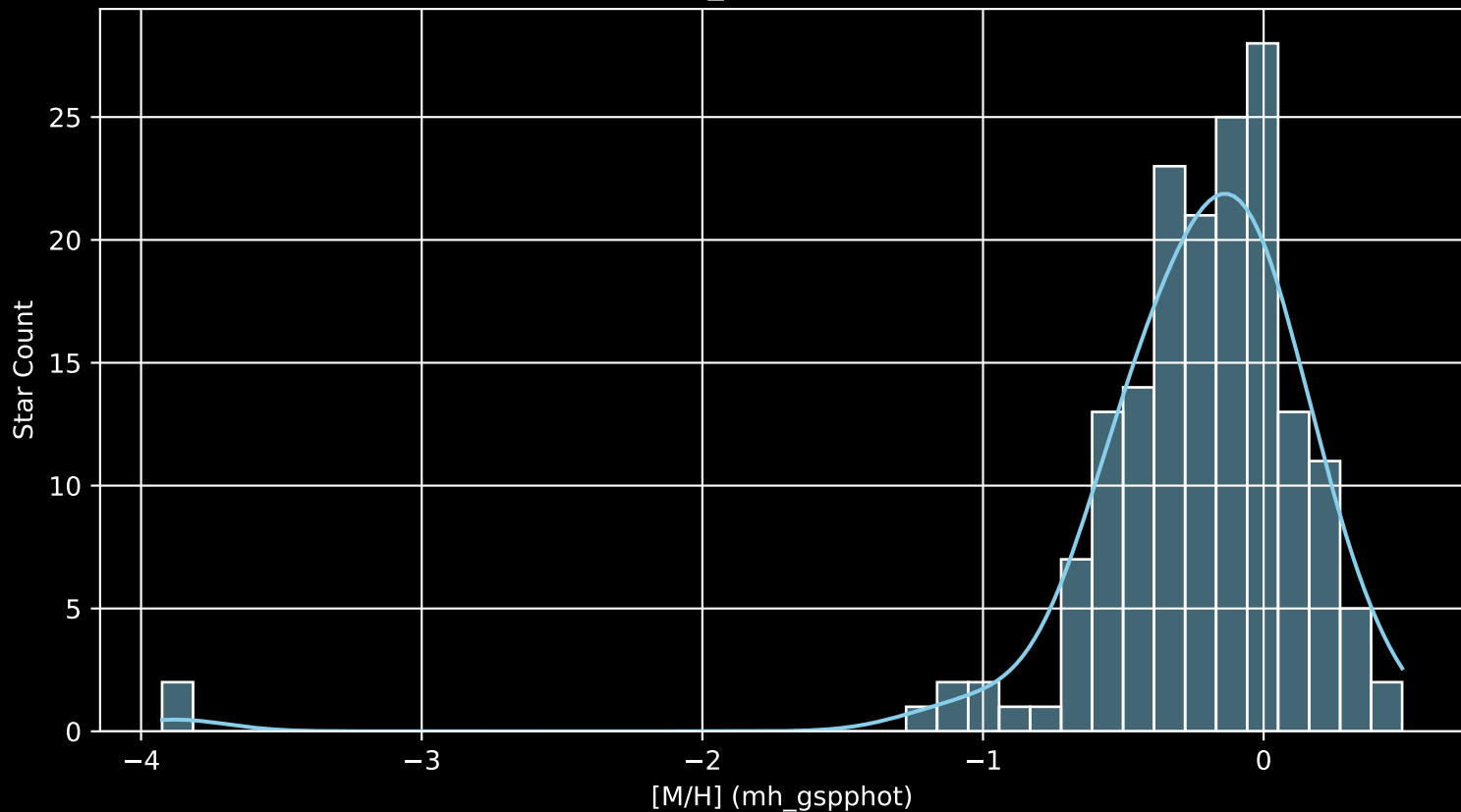
APOGEE DR17 Field: [268-23-O_TESS [M/H] (mh_gspphot) (n= 171)
