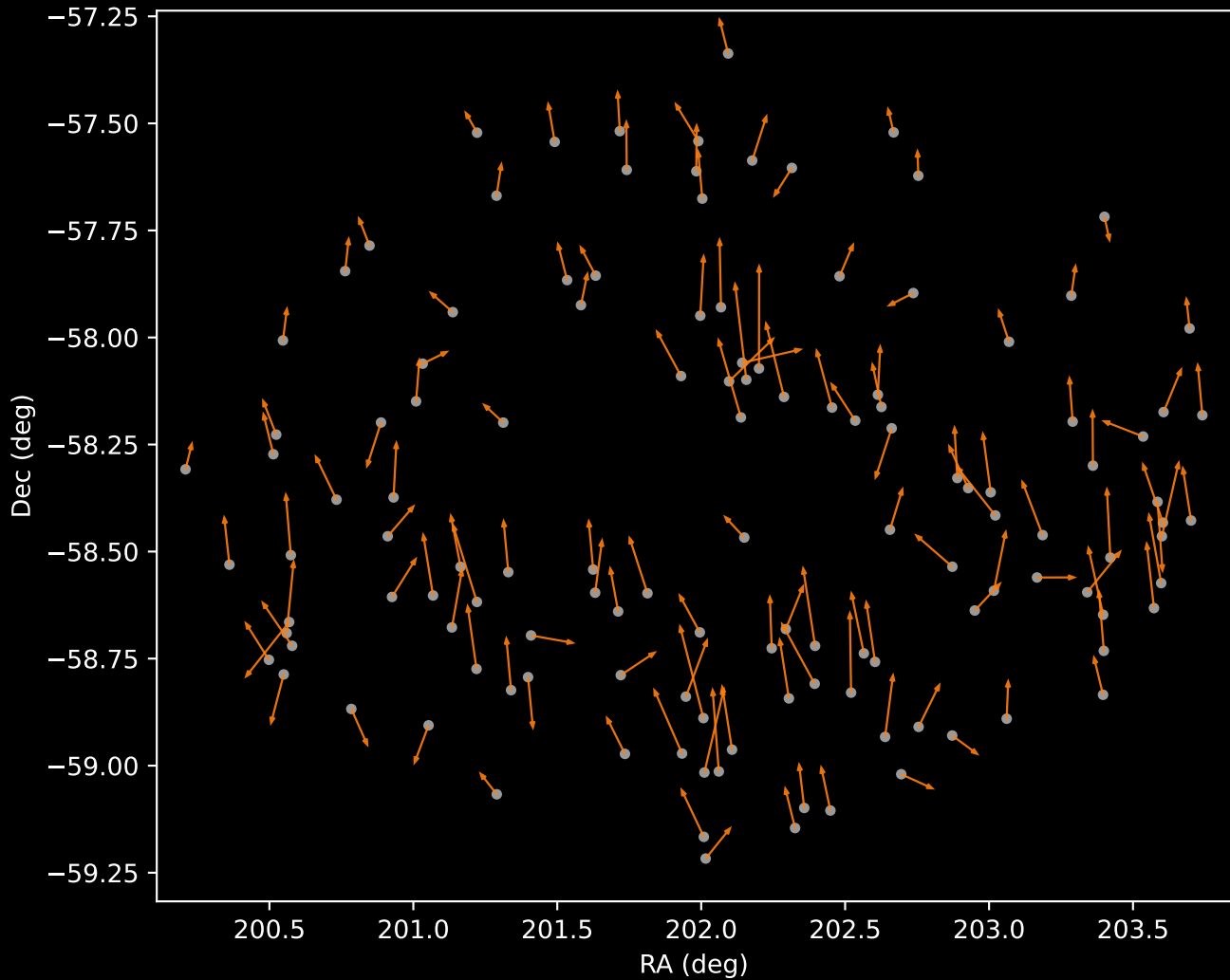
APOGEE DR17 Cluster 2 Proper Motion Vectors (n=128)
