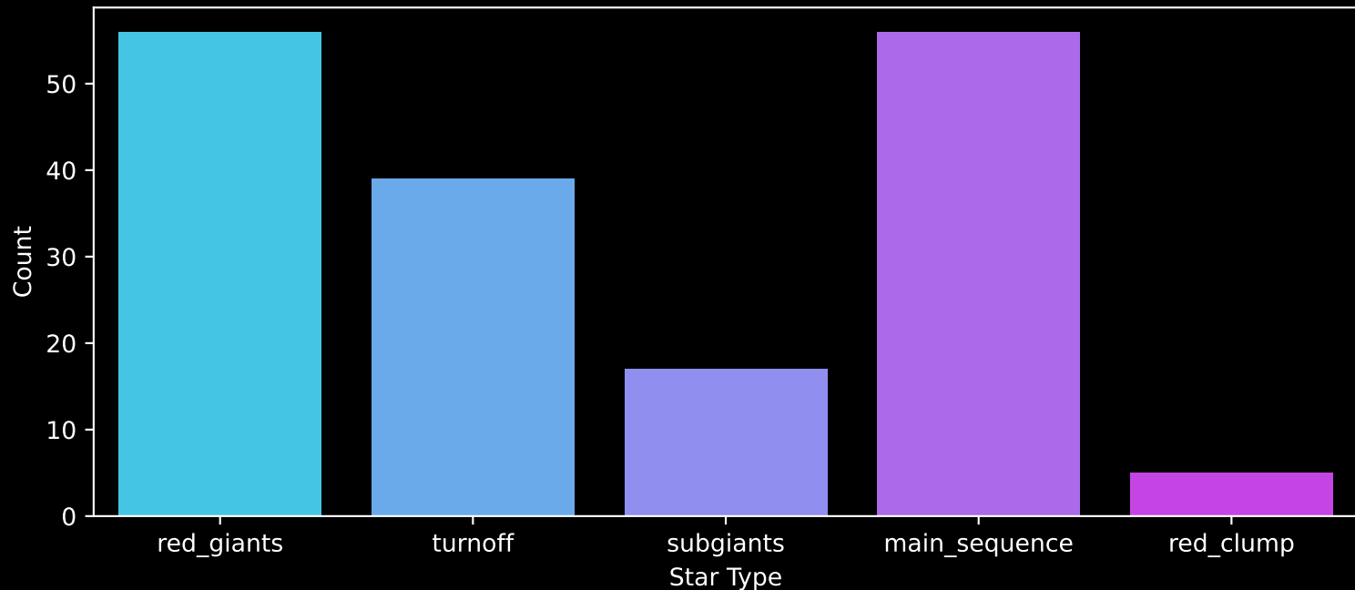
APOGEE DR17 Field: [268-23-O_TESS] Count plot of Star Type
