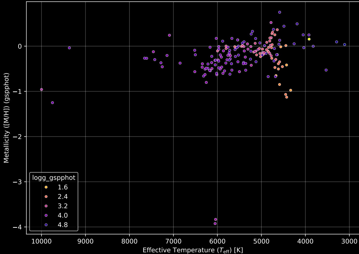
APOGEE DR17 Field: [268-23-O_TESS] Stellar Population Parameters (n= 173)
