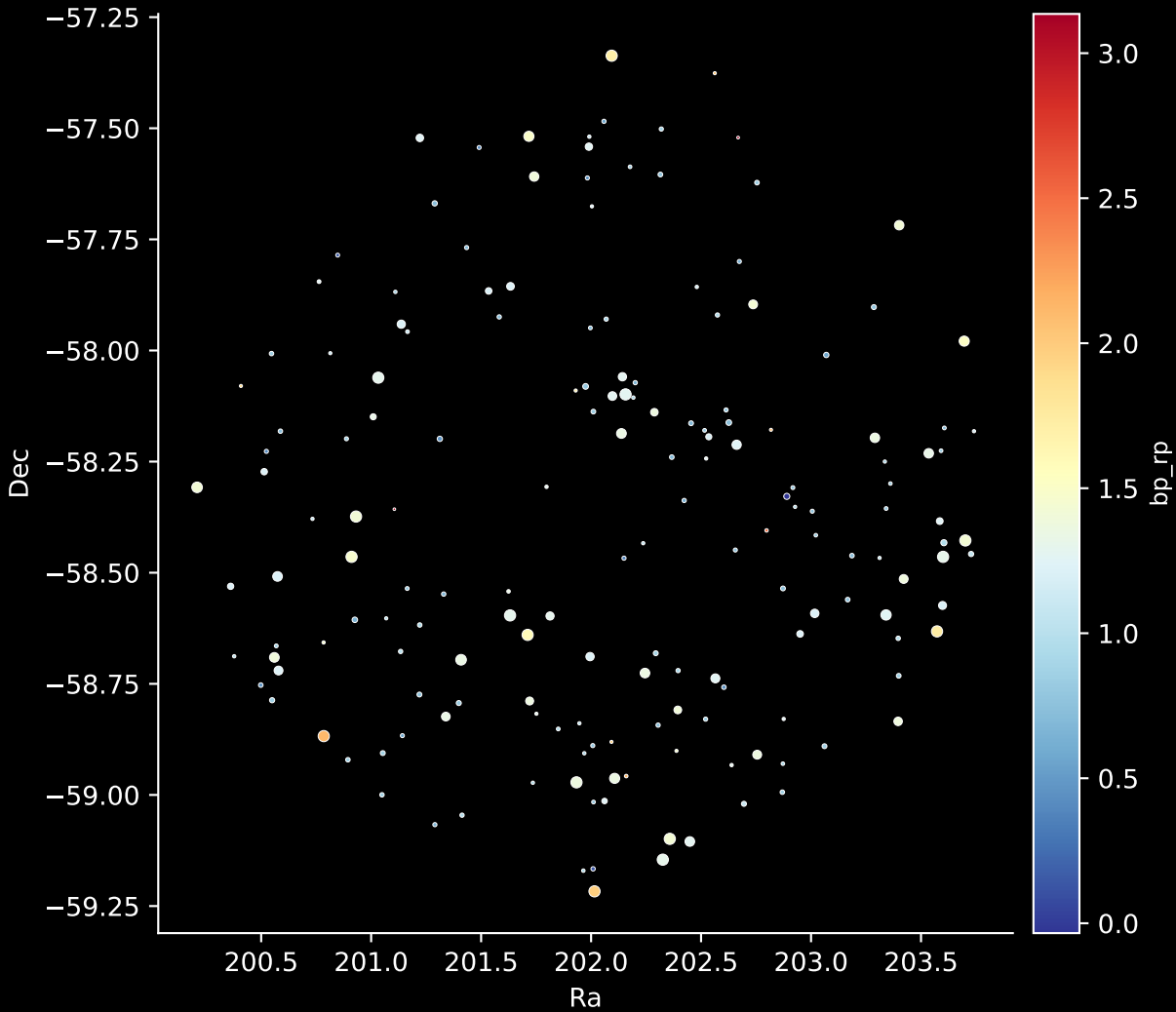
APOGEE DR17 Field: [268-23-O_TESS] Stars: 173
