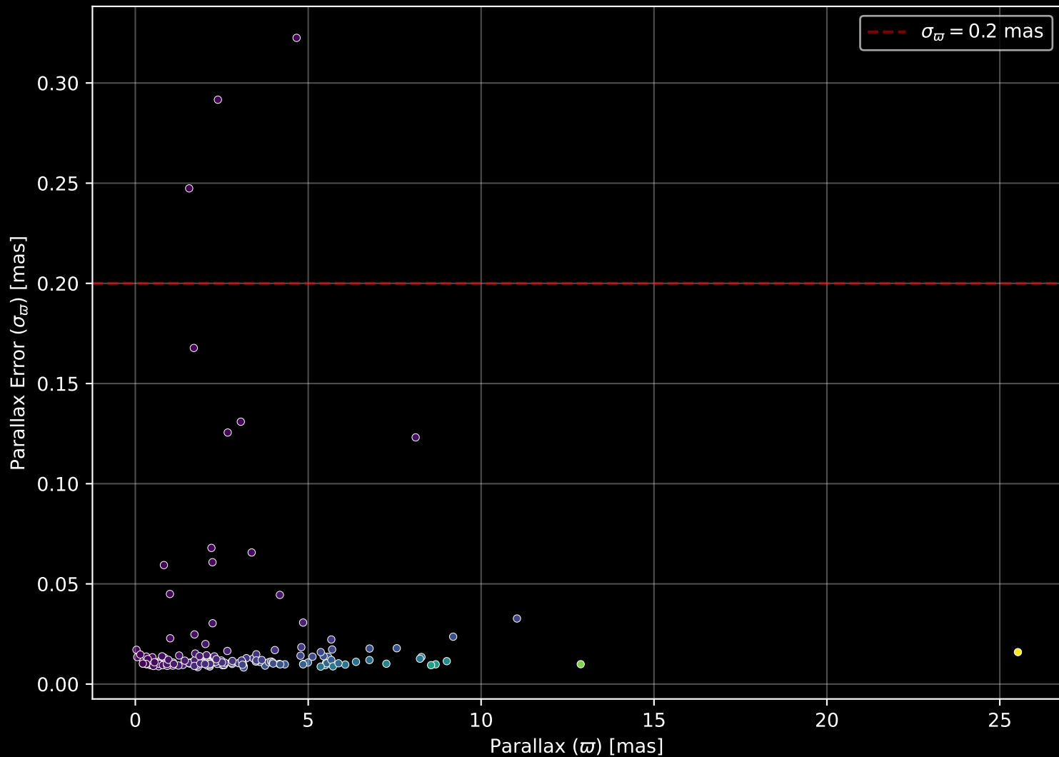
APOGEE DR17 Field: [268-23-O_TESS] Parallax Quality (n= 173)
