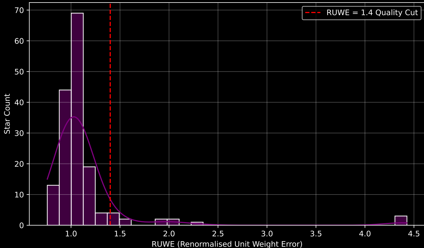
GAPOGEE DR17 Field [268-23-O_TESS] RUWE Distribution (n= 163)
